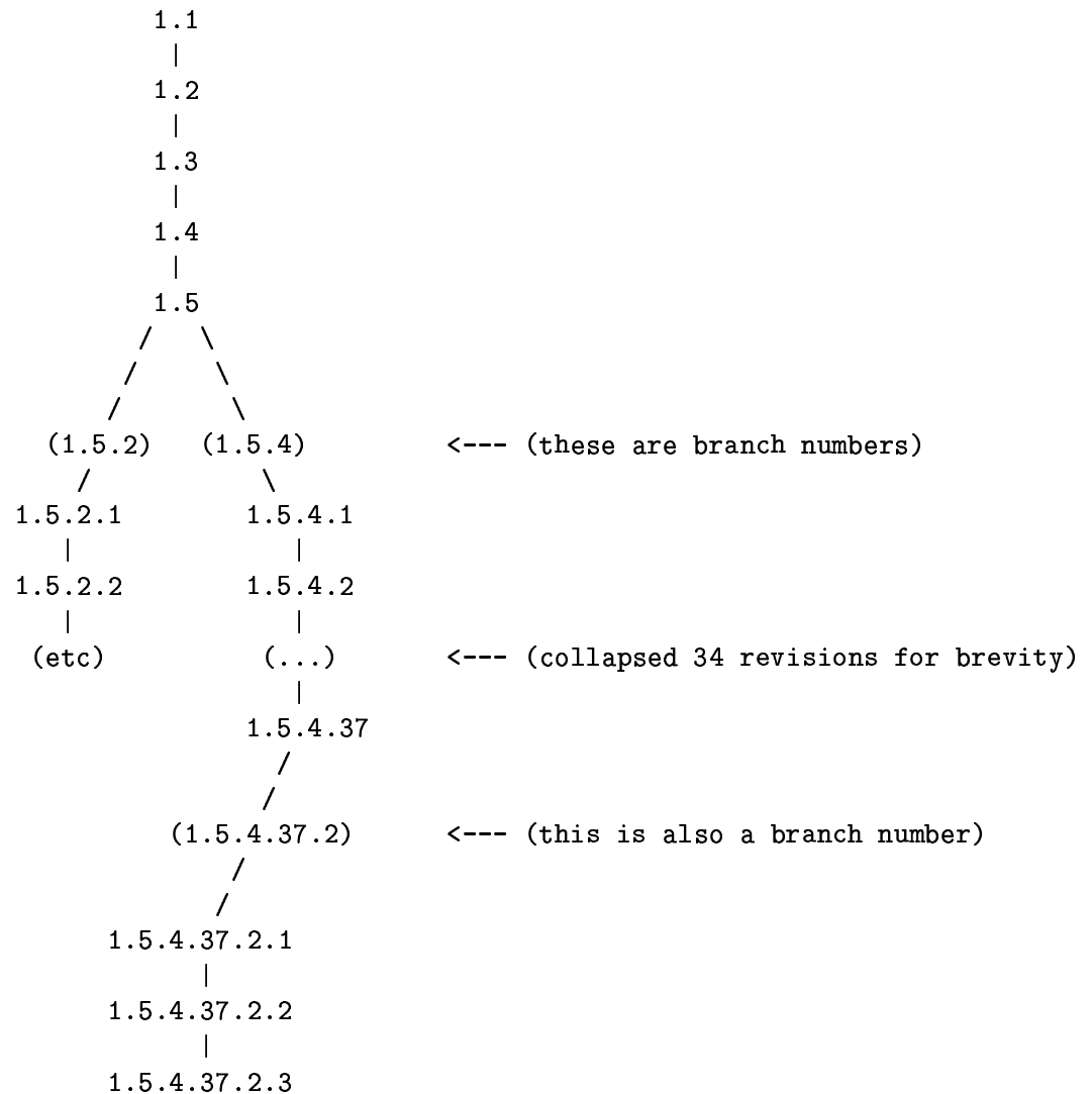
[Figure 2.4: An unusually high degree of branching. Time flows downward.]
