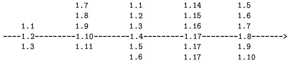
[Figure 2.2: The same tag as a "straight sight" through the revision history.]
