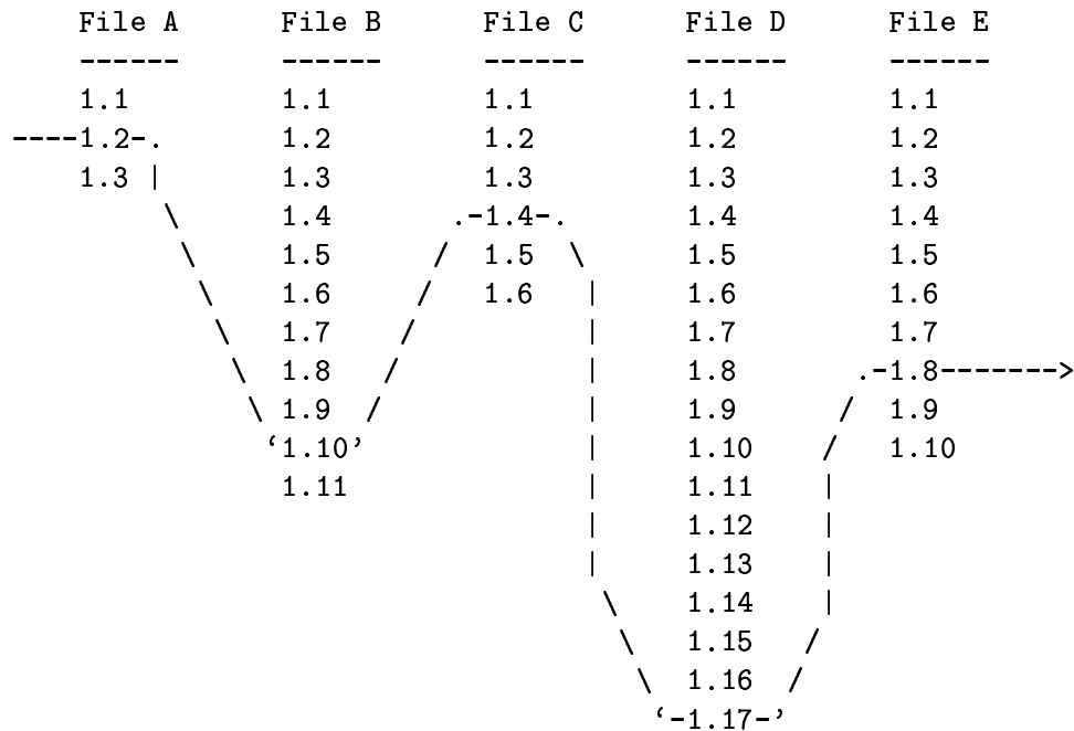
[Figure 2.1: How a tag might stand in relation to files's revisions.]
